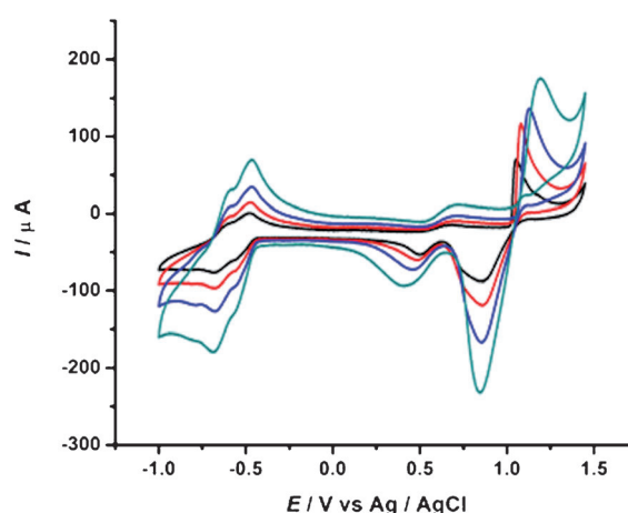
Figure 3. Cyclic voltammograms of 1 ( 2 \times 10^{-3} M) in a pH 3.2 solution (1 M Na 2 SO 4 /H 2 SO 4 ) at scan rates (from inner to outer) of 5, 10, 20, and 50 mVs –1 . The working electrode was glassy carbon (1.5 mm) and the reference electrode was Ag/AgCl.
