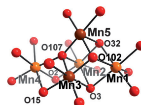
Figure 2. The {Mn 5 O 6 } cubane core of 1 , described as an appended [Mn III 2 Mn II 2 O 4 ] 2+ cubane where Mn1, Mn2, Mn3, Mn5 are connected to manganese atom Mn4 through oxygen atom O107 from the cube and oxygen atoms O2 and O15 of the {SiW 9 } cluster. Mn II orange, Mn III brown, O red.
