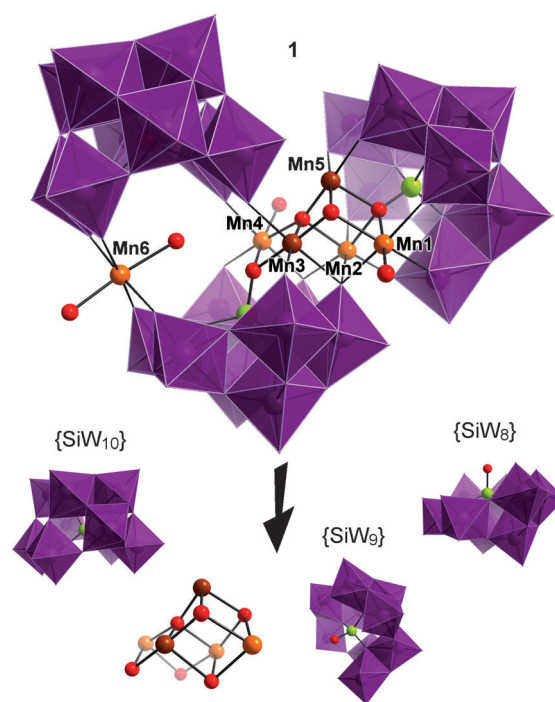
Figure 1. [Mn III 2 Mn II 4 (μ 3 -O) 2 (H 2 O) 4 (B-β-SiW 8 O 31 )(B-β-SiW 9 O 34 )(γ-SiW 10 O 36 )] 18- ( 1a ) showing the three inequivalent silicotungstate Keggin fragments {SiW 8 }, {SiW 9 }, and {SiW 10 } and the appended {Mn 6 O 4 } cubane core with an appended “pendant” Mn ion very similar to that found in the structure of photosystem II. WO 6 purple polyhedra, Mn orange and brown, Si green, O red. Potassium and solvent water molecules have been omitted.
