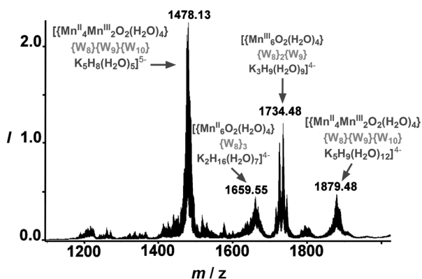
Figure 4. ESI mass spectra of the H 2 O/CH 3 CN solution of 1 . The envelopes of compound 1 and re-organized isostructural species were observed. {W 8 } = {SiW 8 O 31 }, {W 9 } = {SiW 9 O 34 }, and {W 10 } = {SiW 10 O 36 }.
